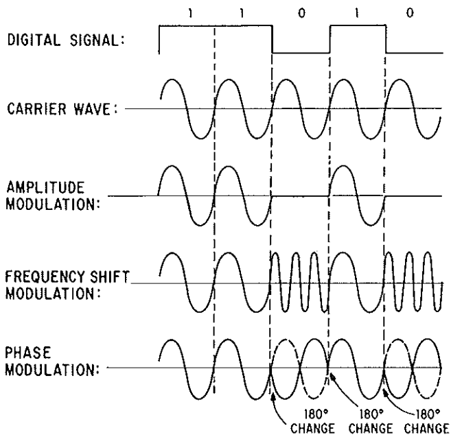
Figure 20. Modulation techniques
