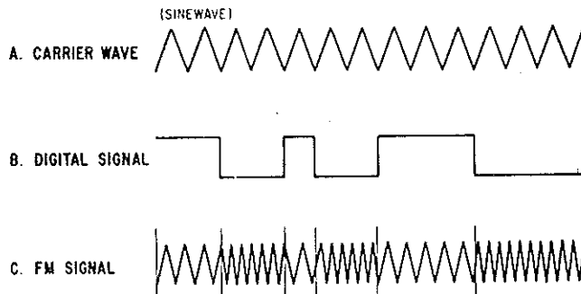
Figure 19. Frequency modulation
