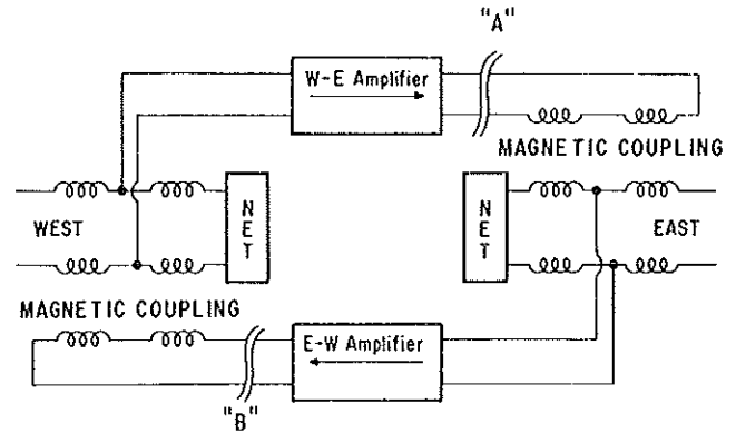
Figure 34. Electromagnetic amplifier connection
