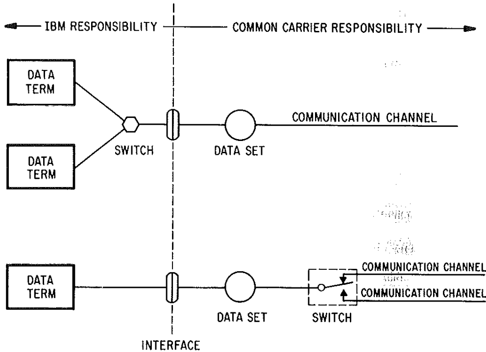
Figure A4.3 Alternate connecting arrangements
