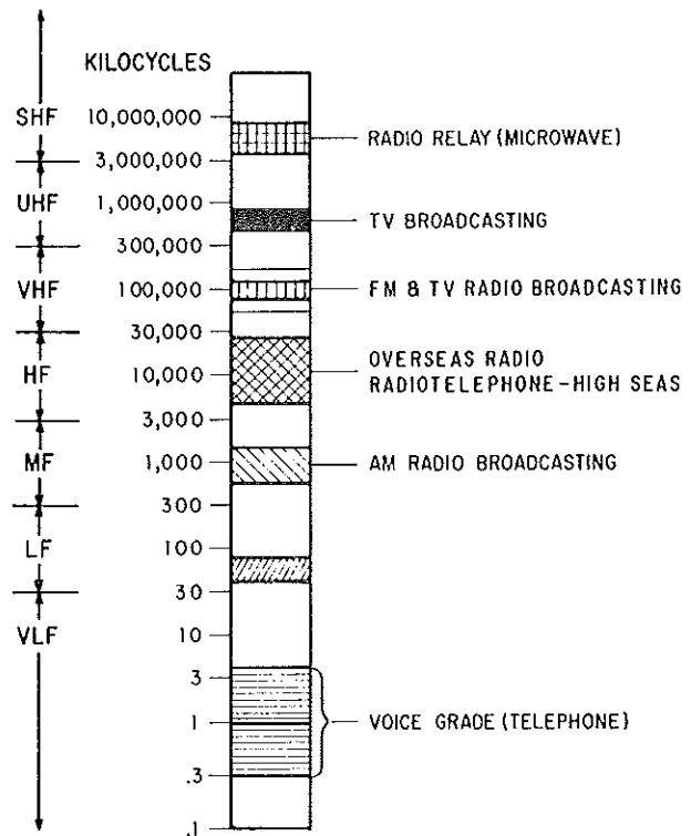
Figure 33. Frequency spectrum
