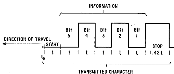
Figure 11. Asynchronous signal
