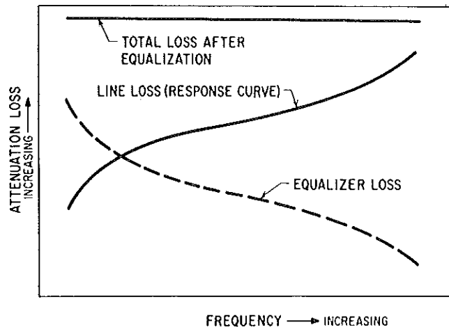
Figure 24. Frequency distortion
