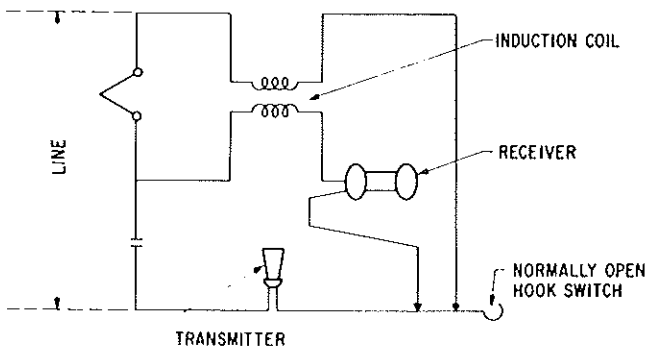
Figure A1.5 Basic common battery subscriber station
