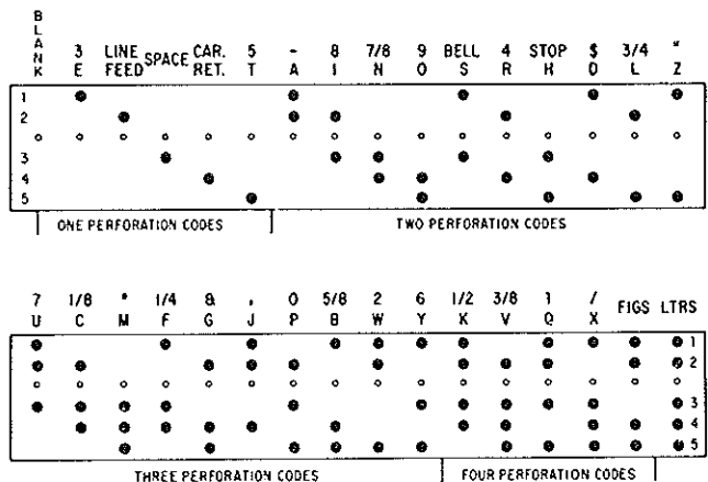
Figure 5. Baudot code
