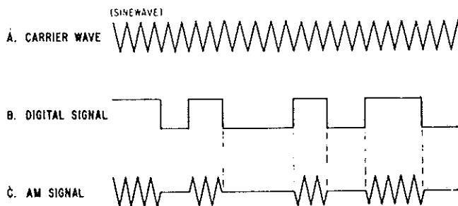
Figure 18. Amplitude modulation
