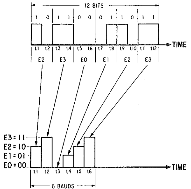
Figure 13. Bauds vs. bits
