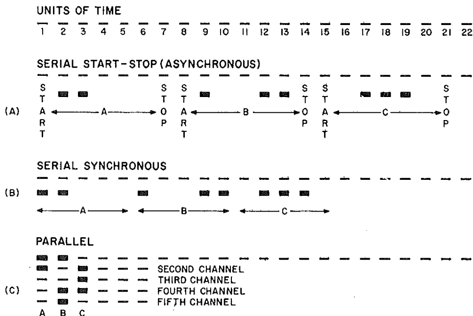
Figure 12. Transmission modes
