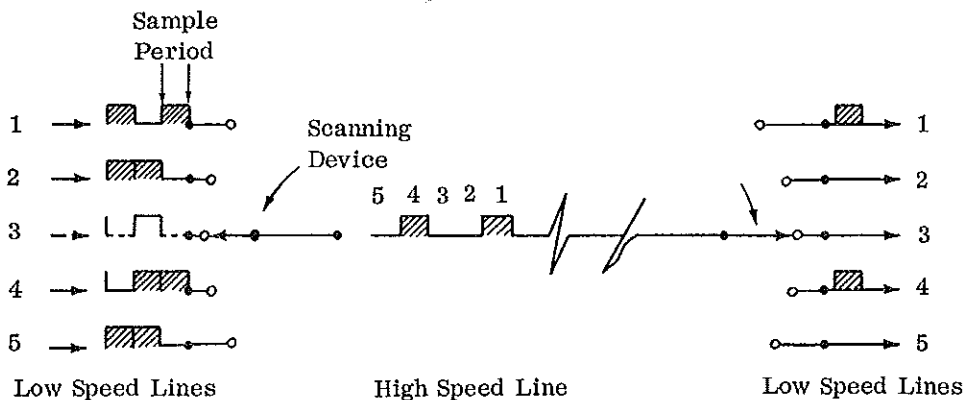
Figure 23. Time multiplexing
