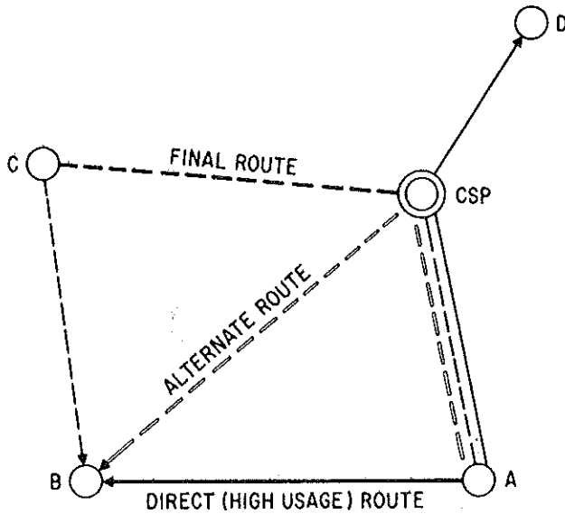
Figure 49. Trunk arrangements
