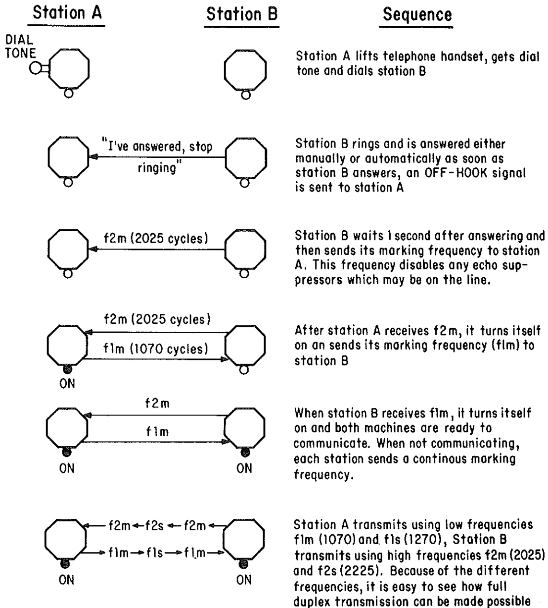
Figure A4.2 Data set handshaking
