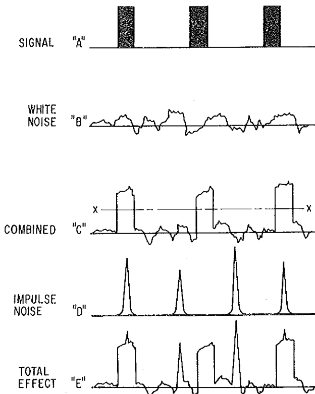
Figure 28. Effect of white noise
