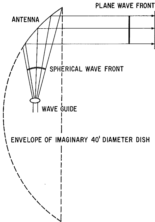
Figure A3.6 Horn-reflector antenna
