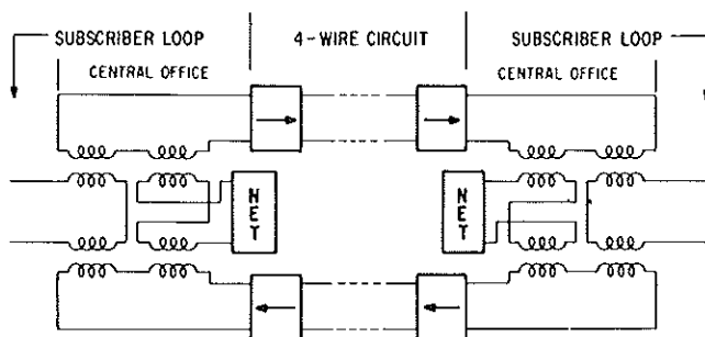
Figure 36. 4-wire circuit with 2-wire termination
