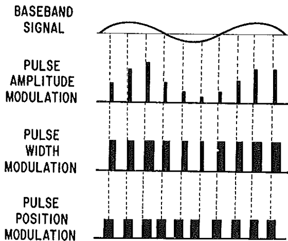
Figure 21. Pulse modulation methods
