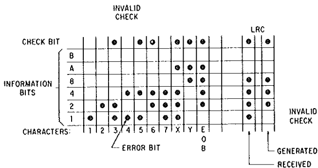
Figure 30. Error correction
